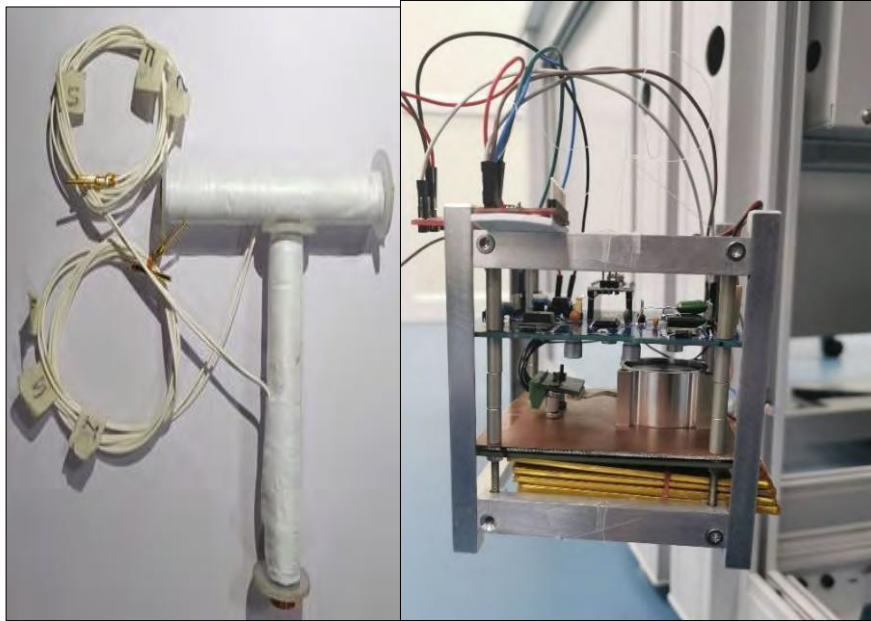
Figure: Magnetotorquesr and Single axis Momentum wheel based ADCS system developed at IIST by M.Tech. Control Systems students.
